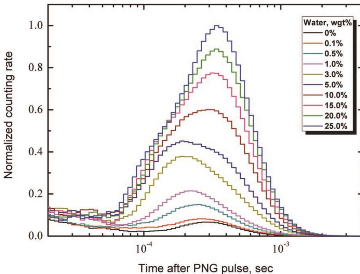
FIG. 3. Die-away curves of thermal neutrons as modeled in the DAN-DE detectors for a homogeneous model of regolith with different water contents (by % weight faction). Black corresponds to 0% of water weight; red, 0.1% water weight; dark cyan, 0.5% water weight; magenta, 1.0% water weight; dark yellow, 3.0% water weight; navy blue, 5.0% water weight; wine, 10% water weight; pink, 15% water weight; olive green, 20% water weight; blue, 25% water weight. All counting rates are normalized to the counting rates in the detector of thermal neutrons for the soil with 25% water weight (the maximum of this curve corresponds to the counting rate 10^6 counts/s/time bin).
