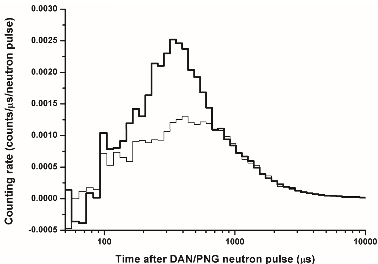
FIG. 4. The comparison between die-away curves (thermal neutrons) gathered for relatively dry soil (3–5% by weight fraction), shown as a thin line, and dry soil with a “water spot” under the rover (thin polyethylene layer with radius <50 cm on top of the surface under the rover), shown as a bold line.
